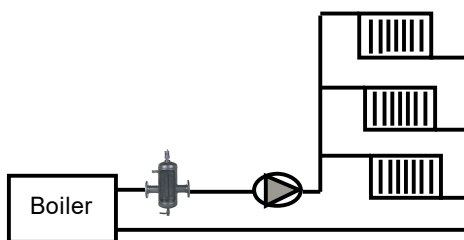
Heating System
